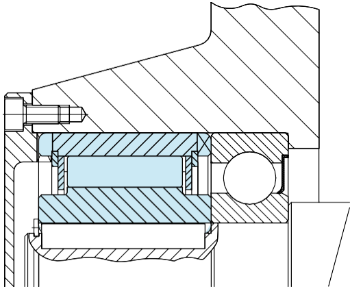
Figure 3: Mounting NF
