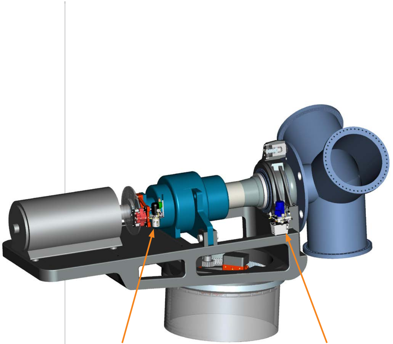
Stand alone hydraulic power unit for active rotor brake control
