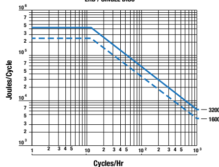
HEAT DISSIPATION ERD / SINGLE DISC
