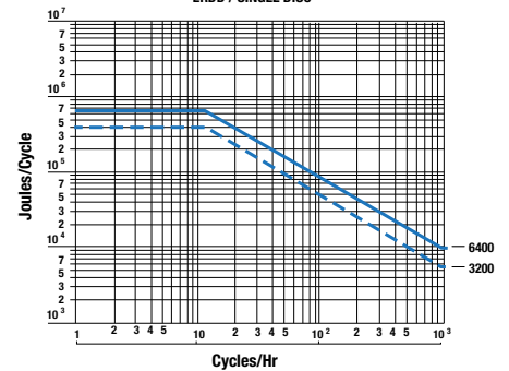
HEAT DISSIPATION ERDD / SINGLE DISC
